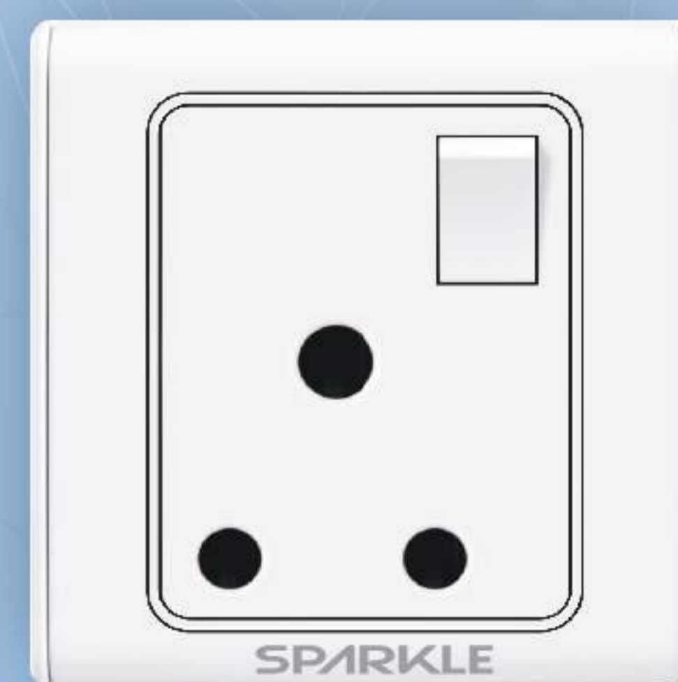
15A 3 PIN SKT WITH SW (15A, 250V~)
